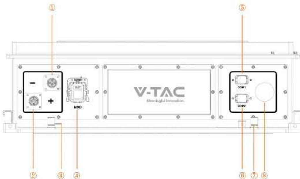
Figure2-5 Structure layout
