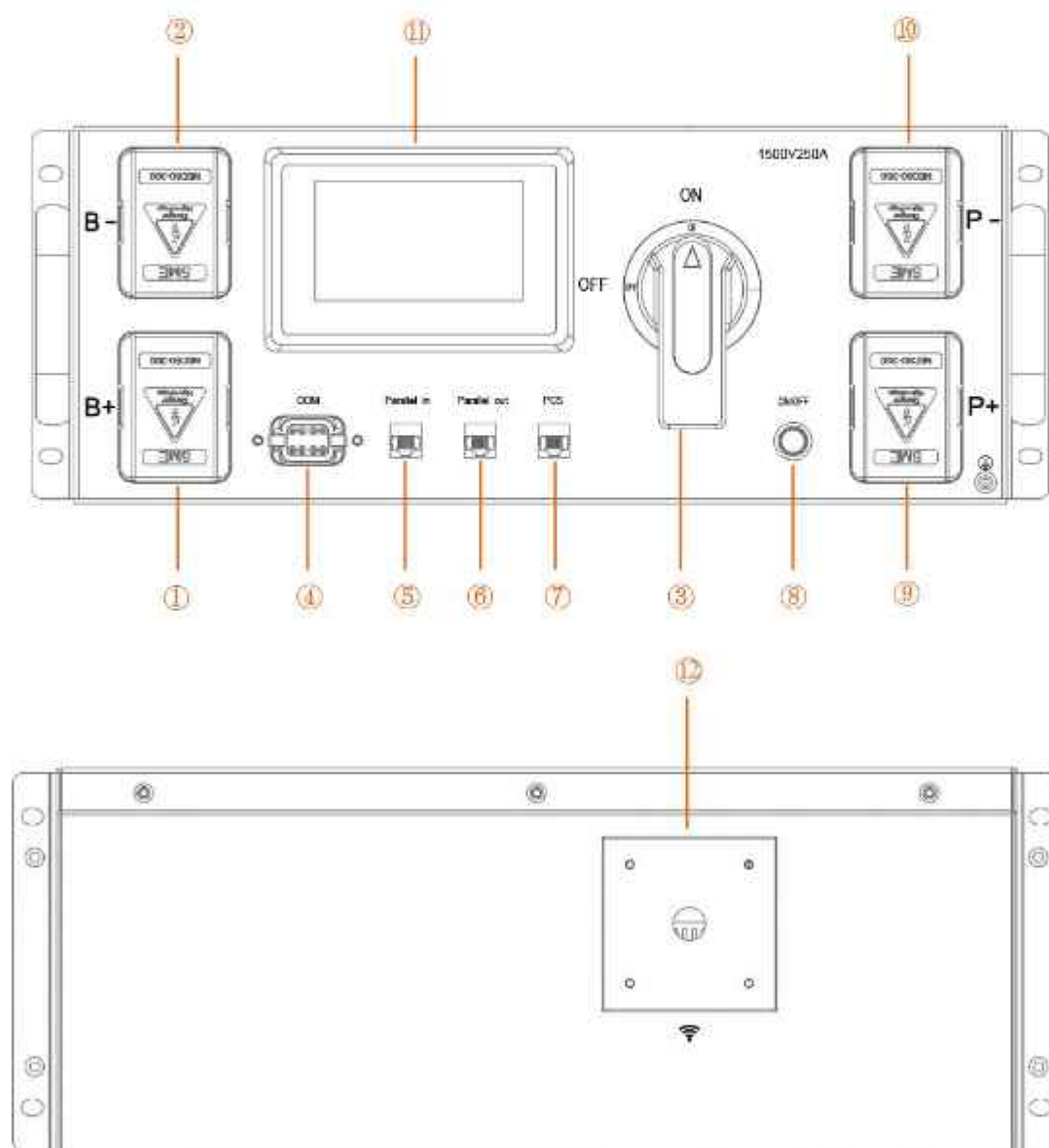
Figure2-6 Structure layout
